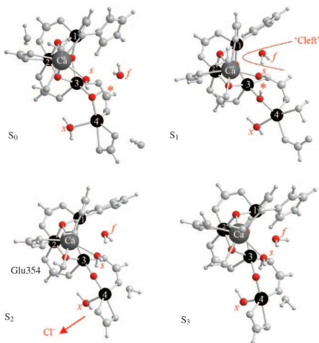
Figure 3. Heptahydrated \text{II}^{\text{a}} , \text{IIa}^0 , \text{II}^+ , and \text{II}^{+*} species corresponding to calculated WOC structures in S_0 to S_3 with metal atoms, oxo bridges, and “important” water ligands highlighted. Mn atoms are labeled 1 to 4. Water ligands labeled “f” and “s” correspond to “fast” and “slow” exchanging substrate waters. “x” denotes the water ligand tentatively identified in the latest 2.9 Å XRD structure. Protonated oxo bridge denoted by asterisk. “Cleft” region, Glu354 equivalent residue, and approximate location of XRD-identified chloride are also shown.
